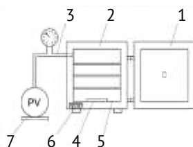
Figure 1. The laboratory installation used to torrefact biomass samples in vacuum
