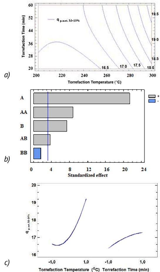
Figure 2. Calorific value of the biomass mixture that includes 50% of blackberry, 50% of sea buckthorn according to torrefaction temperature and time: a) Contours of Estimated Response Surface; b) Standardized Pareto Chart for q_{p,net, M=10\%} (A – Torrefaction temperature, ^\circ\text{C} ; B – Torrefaction Time, min); c) Main Effect Plot for q_{p,net, M=10\%} of thermal regimes; 7 – the vacuum pump.
